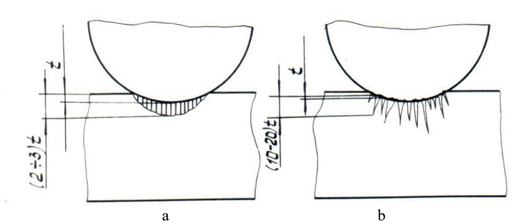
Figure 1 – Scheme of stress fields at rock fracture by tungsten carbide plates (a) and PSHM (b)
