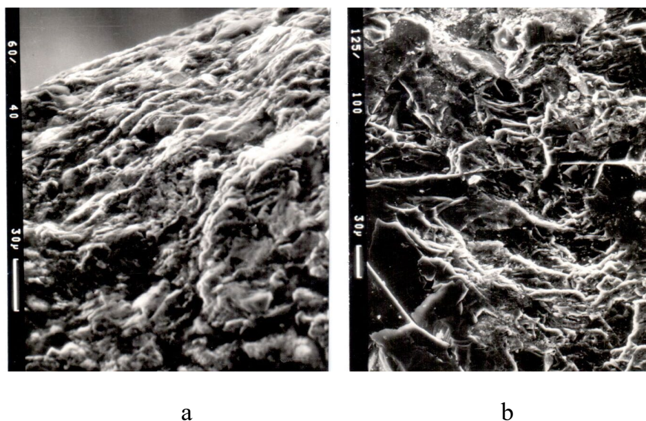
Figure 3 – Microrelief of the cutting surface of the working PSHM with grain size of initial grinding powders 60/40 (a) and 125/100 (b)
